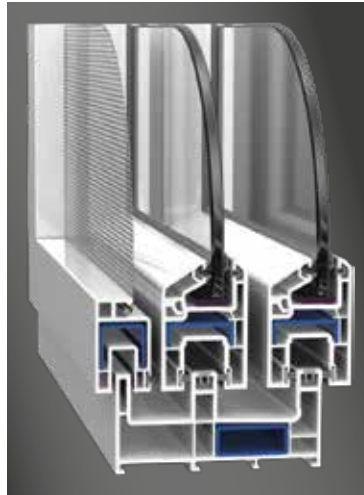
Double Rail with Screen Sash
