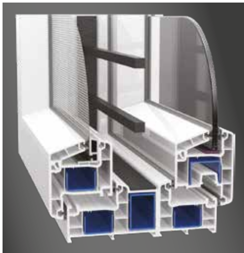
Casement Window with Grill and Mesh
