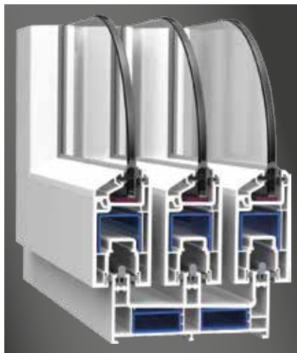
3-Track 3-Panel Door
